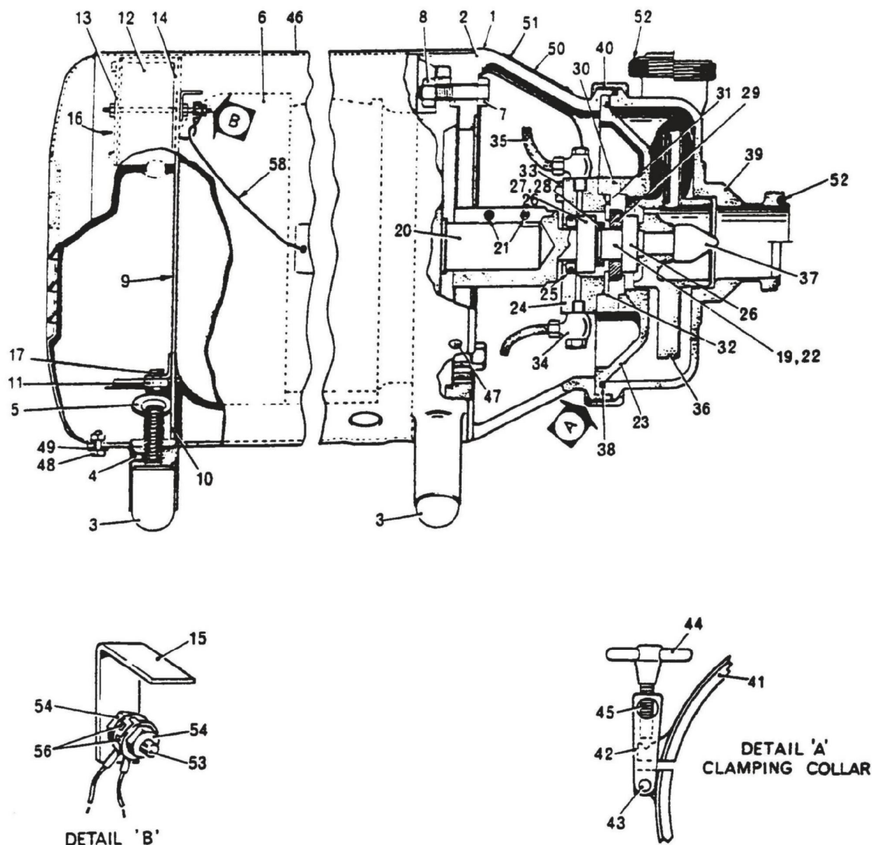
Pump assembly (Series IV)
