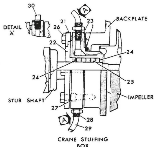
Seal Arrangements (Series IV)
