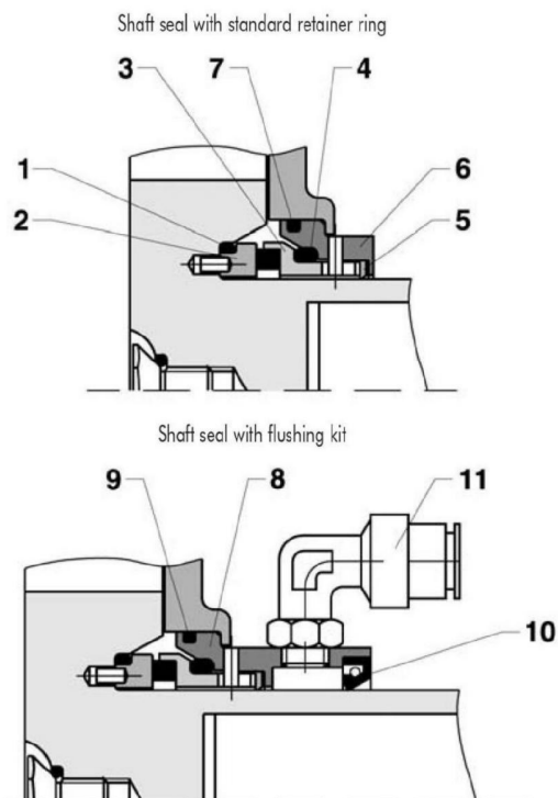
Shaft seal
