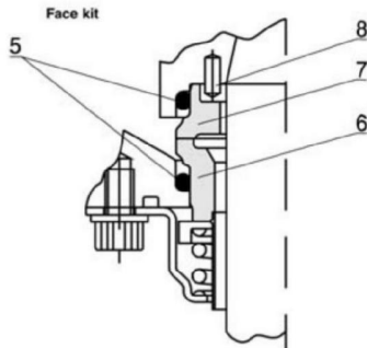
Face kit
