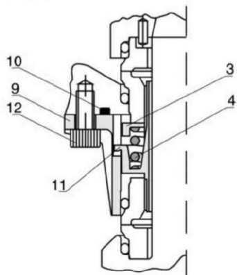
Fixing kit
