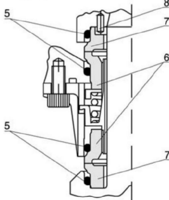
Face kit
